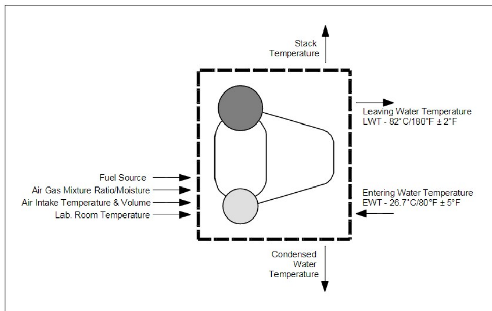
Figure-1. Boiler Steady State Test Controlled Parameters
